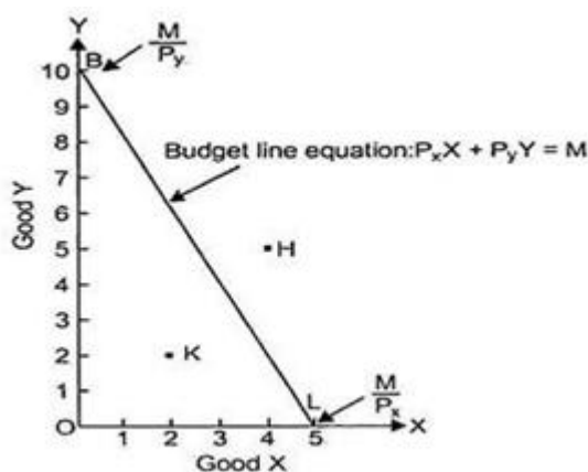
Fig. 2.2.4 Budget Line
