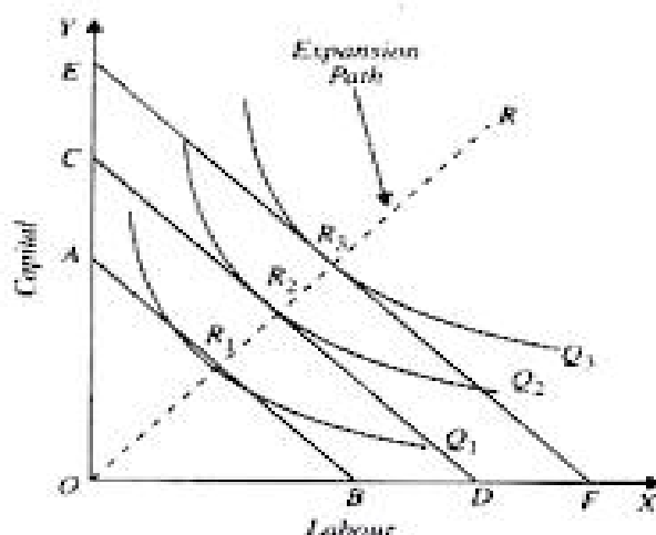
Fig. 3.1.6 Expansion path
